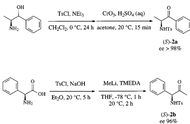
Scheme 3. Synthesis of authentic samples of ( S )- 2a and ( S )- 2b
