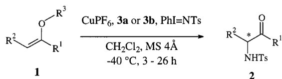
Scheme 2. Copper-catalyzed asymmetric amination of enol derivatives 1
