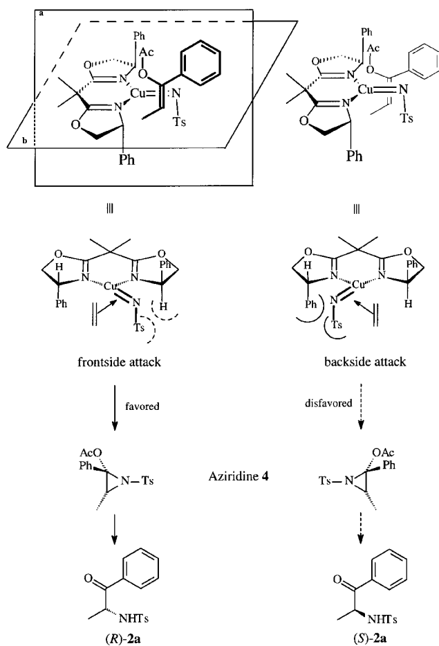
Figure 1. Proposed trajectories for the approach of enol acetate 1aδ in asymmetric aziridination with the catalyst system \text{CuPF}_6/\mathbf{3b} ; plane a relates to the substrate and plane b to the bis(oxazoline) complex.
